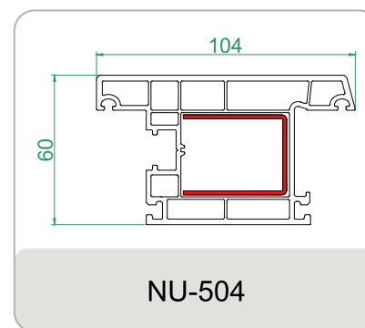
CASEMENT OUTWARD OPENING DOOR SASH 104X60 MM
