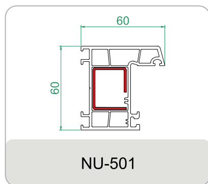
CASEMENT WINDOW OUTER FRAME 60X60 MM
