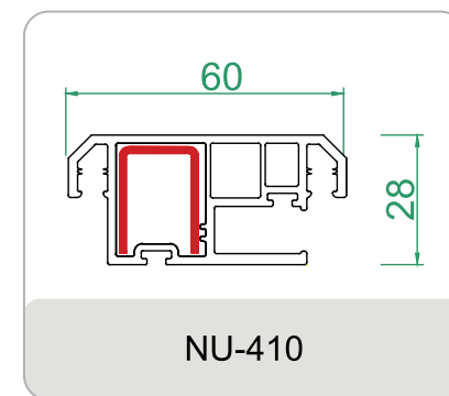
SLIDING WINDOW/DOOR MESH
