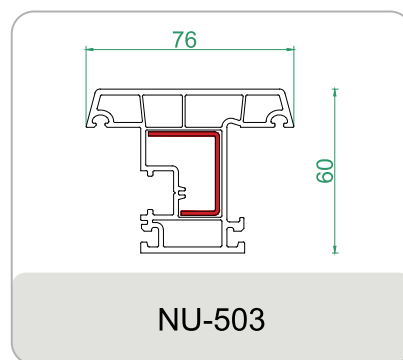
CASEMENT OUTWARD OPENING WINDOW SASH 76X60 MM
