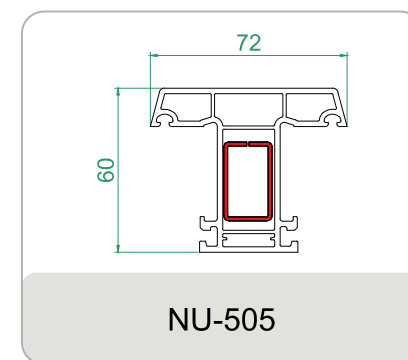
CASEMENT T- MULLION 72X60 MM
