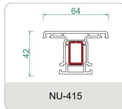
SASH MULLION
