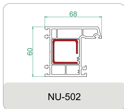
CASEMENT OUTER FRAME 68X60 MM
