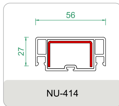
MESH MULLION
